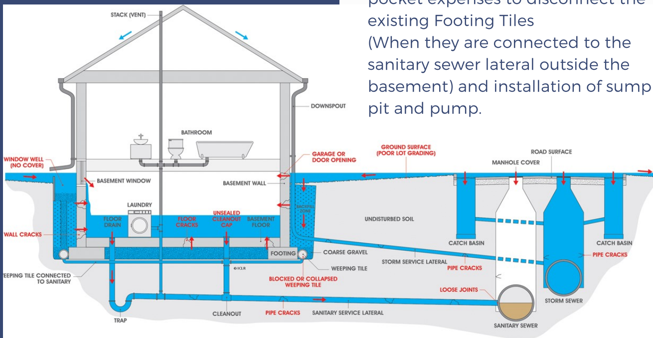
Figure 1 (Below) Flooding caused by foundation draining failure (Source: Handbook for Reducing Basement Flooding, ICLR, 2009)
