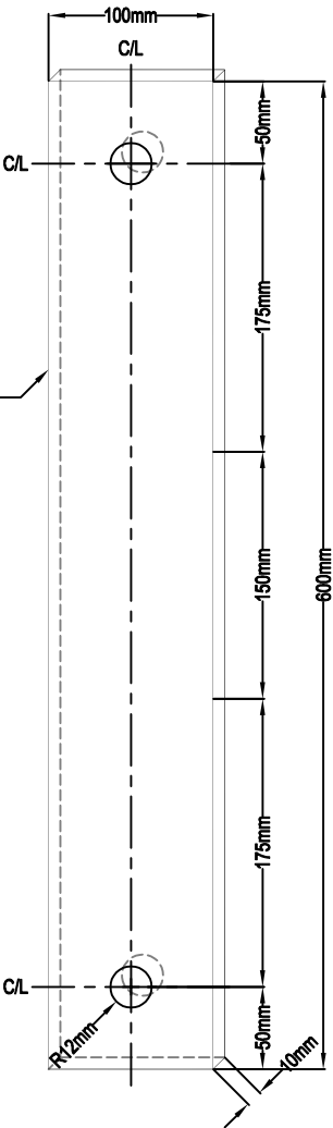
FROST STRAP ANCHORED TO INTERNAL CHAMBER WALL
