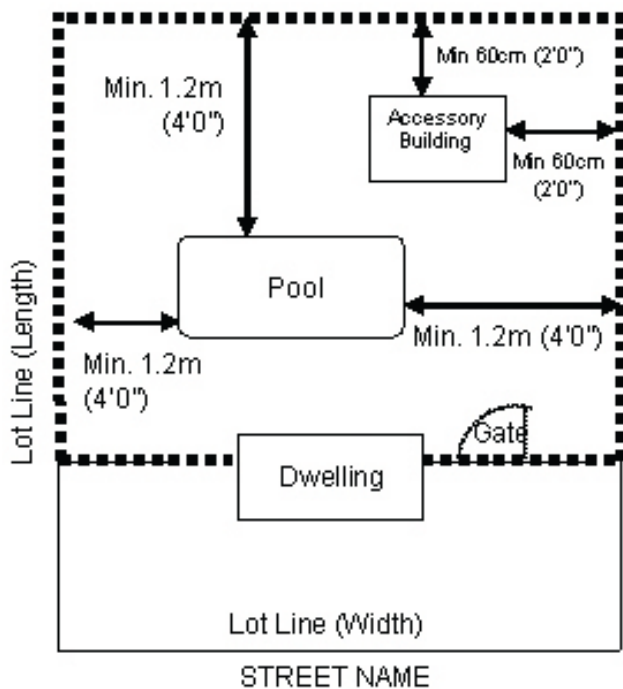
Sample Site Plan Drawing
